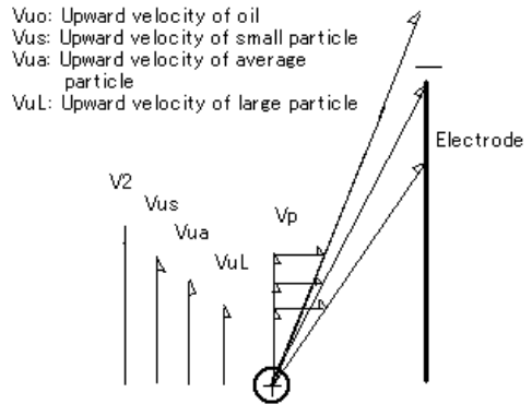
Figure 2 Schematic Figure Showing the Motion of a Positively Charged Particle in a Uniform Electric Field
