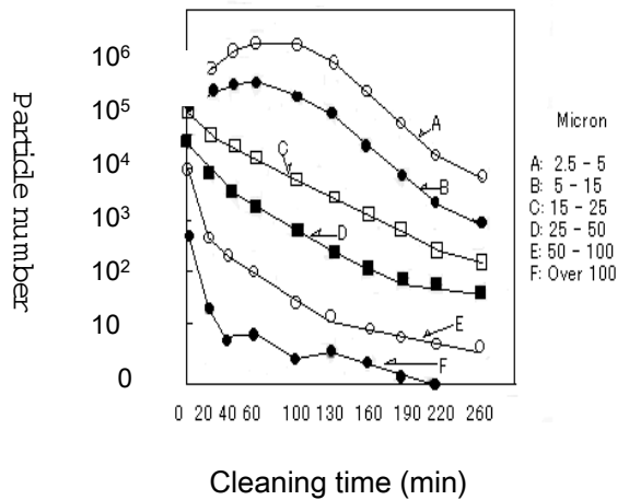
Figure 5 Change of Particle Numbers During Cleaning by an Electrostatic Oil Cleaner
